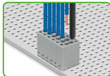
Conductor removal (2080 Series) - via push-button and 1 mm \varnothing operating tool (206-880).
